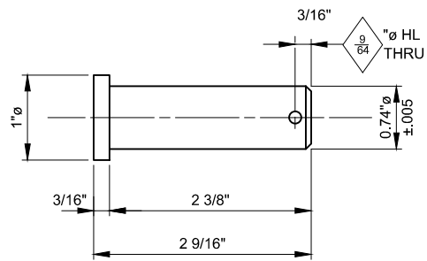
HINGE PIN - Pc. # 6 BRASS
