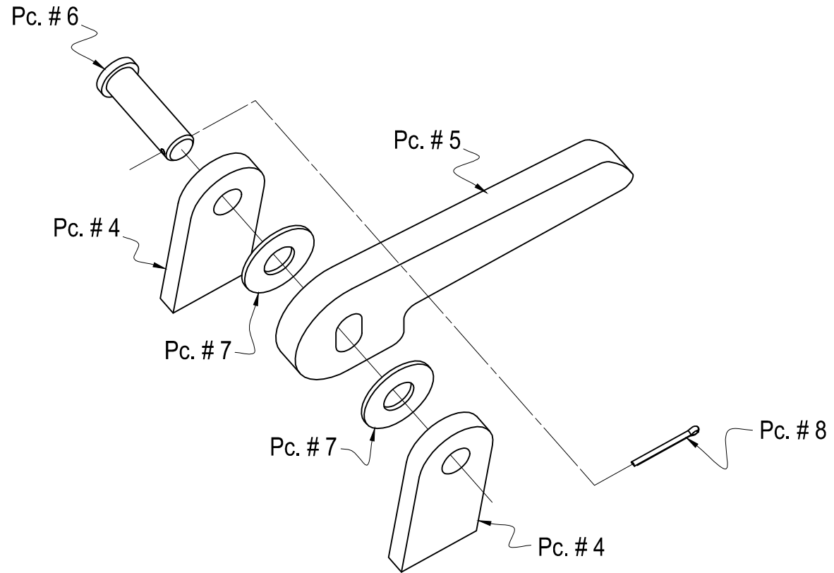
HINGE ASSEMBLY SET PART # DH100
