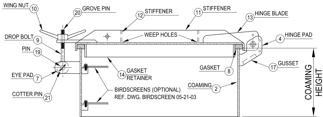
SECTION
