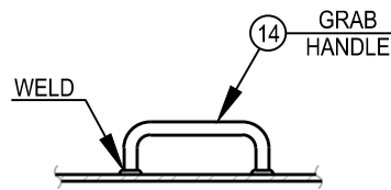
DETAIL OF GRAB HANDLE
